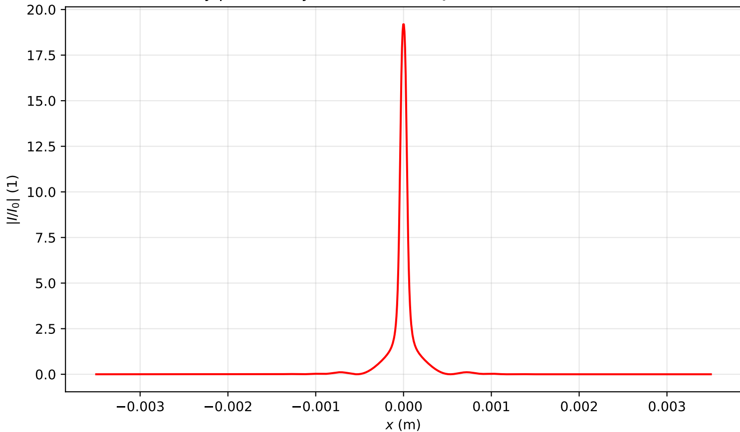
Intensity profile I(x, y = 0, z = 0.955)/I_0 , P_{in}=5.5P_{cr} , artificial time
